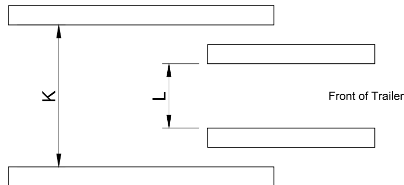
Timber Bunk Positions of existing trailer
